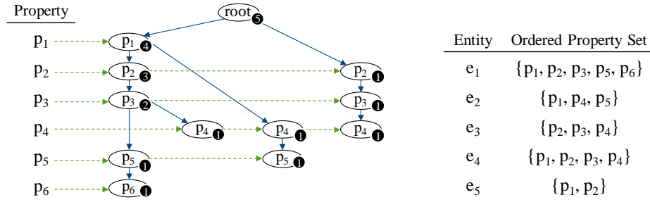
Fig. 1. The SchemaTree derived from the property sets depicted on the right.
